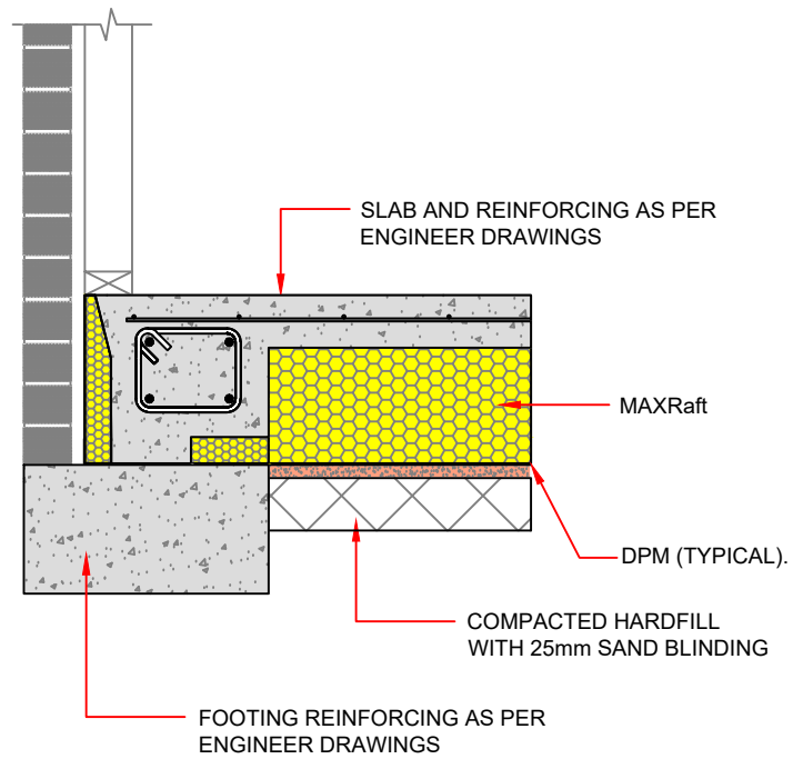
MAXRaft BRICK TO FOOTING DETAIL
